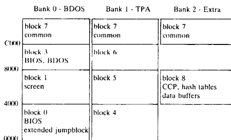
Figure 1a PCW 8256/8512
