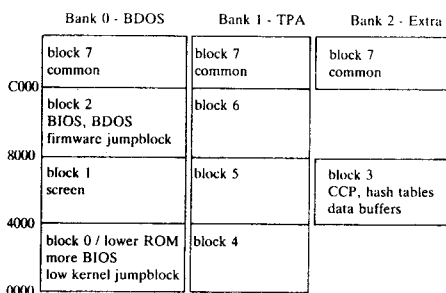
Figure 1b CPC 6128
